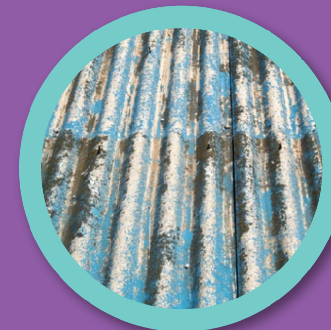
BLUE (CROCIDOLITE)
